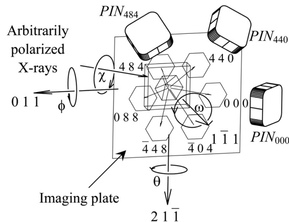
図 L.6 A schematic drawing of the goniometer on which the sample crystal was mounted (reproduction of Fig. 7 in Okitsu et al. (2006)) [49].
