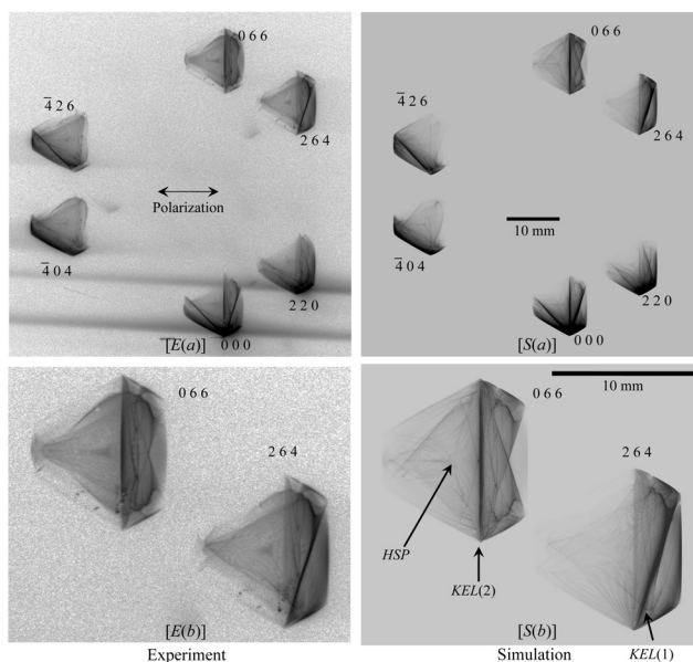
図 L.12 [E(a)] and [S(a)] are experimentally obtained and computer-simulated six-beam X-ray pinhole topographs with an incidence of horizontal-linearly polarized X-rays with a photon energy of 18.245 keV. [E(b)] and [S(b)] are 0 6 6 and 2 6 4 reflected X-ray images enlarged from [E(a)] and [S(a)] (reproduction of Fig. 9 in Okitsu et al. (2012) [50]).
