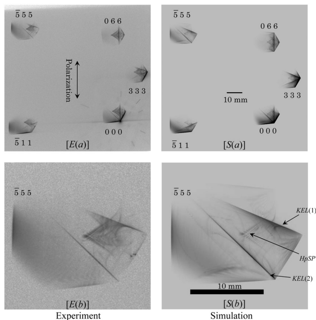
図 L.11 [E(a)] and [S(a)] are experimentally obtained and computer-simulated five-beam X-ray pinhole topographs with an incidence of vertical-linearly polarized X-rays whose photon energy was 18.245 keV. [E(b)] and [S(b)] are \bar{5} 5 5 reflected X-ray images enlarged from [E(a)] and [S(a)] (reproduction of Fig. 8 in Okitsu et al. (2012) [50]).
